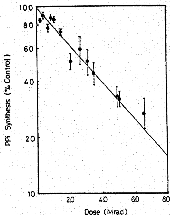
Fig. 3. Radiation inactivation of acid-base induced \text{PP}_i synthesis by chromatophores of Rhodospirillum rubrum . The irradiation of chromatophores and the reaction conditions of acid-base induced \text{PP}_i synthesis were as described in section 2. All data points are means of at least 3 assays with line fitted by regression analysis ( r = 0.95 ). The intersect on the line at 37% activity of control gives the D_{37} dose value. The control activity of \text{PP}_i synthesis was 98 nmol \text{PP}_i formed/mg BChl/min.
