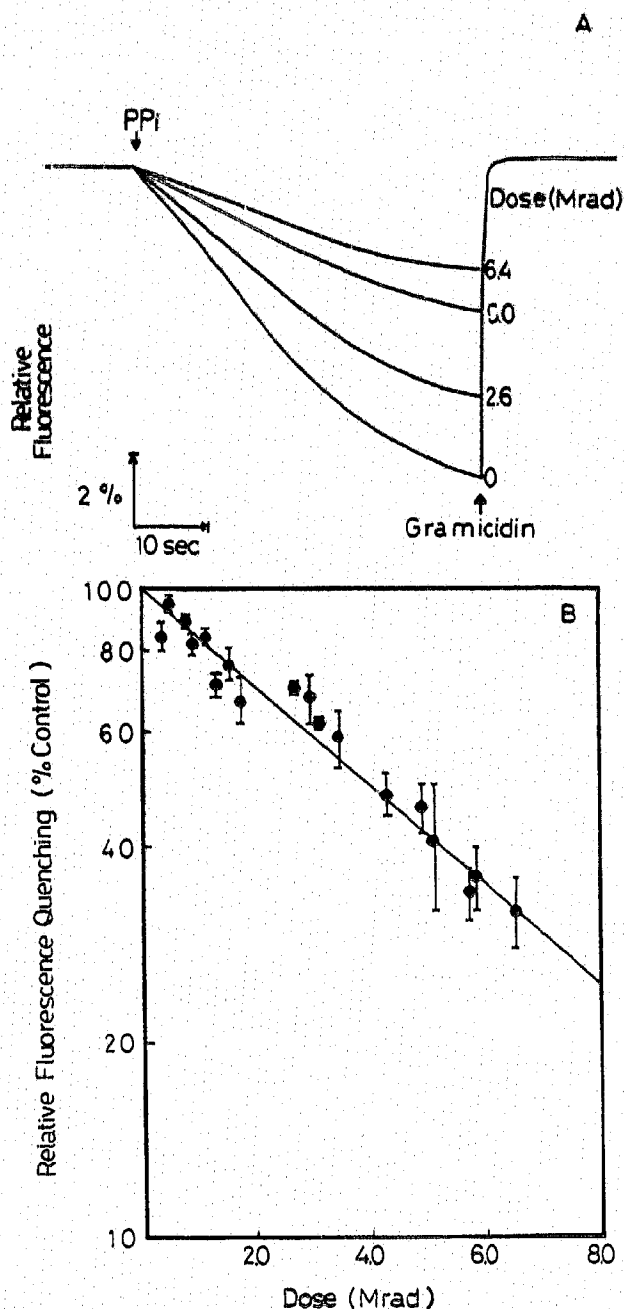
Fig. 2. Radiation inactivation of \text{PP}_i -mediated \text{H}^+ -translocation of chromatophores from Rhodospirillum rubrum . The irradiation of chromatophores and the measurement of \text{H}^+ -translocation were carried out as described in section 2. The initial rates of fluorescence quenching were determined from changes in fluorescence observed in first 30 s (A). One percent of fluorescence quenching represents 0.16 nmol proton influx determined by the direct titration of standard HCl. The data points in (B) are the means of at least 3 assays with the line fitted by regression analysis ( r = 0.95 ). The line of intersect at 37% of control activity gives the D_{37} dose value.
